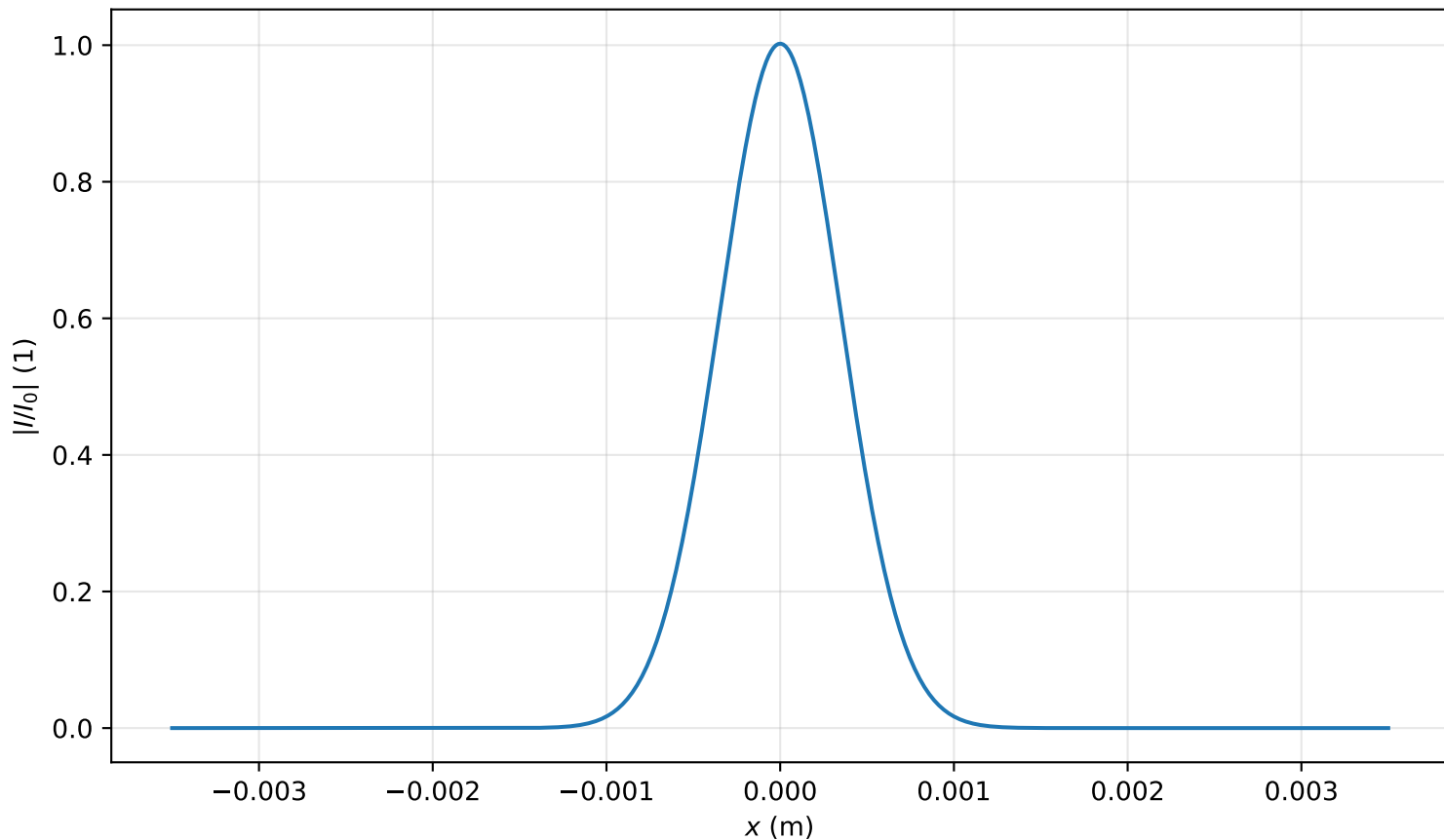
Intensity profile I(x, y = 0, z = 0.080m)/I_0 , P_{in}=0.6P_{cr} , artificial time
